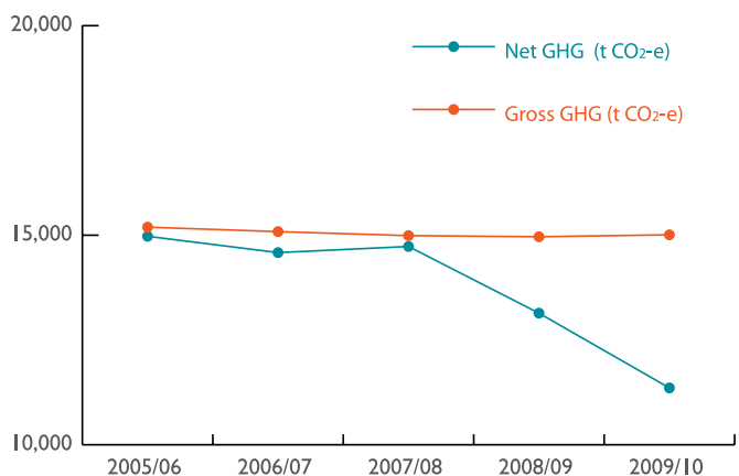
Figure 2: Absolute emissions, 2006-2010
